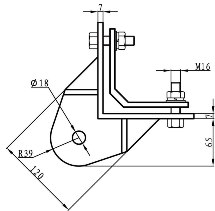
Clevis for Corner Tower 耐张塔用紧固夹具
